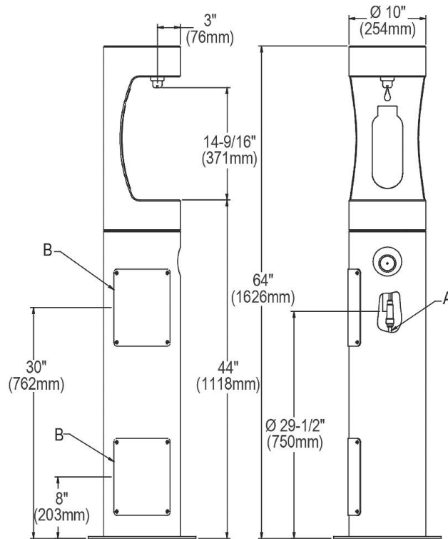
SIDE & FRONT VIEWS
